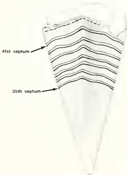
TEXT-FIG. 4. Camera-lucida drawing of the oral part of C.46812, Conoteuthis dupiniana d'Orbigny, 1842 reproduced in Pl. 21, fig. 2A-H. Dorsal view, \times 12 . This drawing supplements that of text-fig. 3 and illustrates the rapid transformation of Diplobelus -like mid-dorsal saddles of the suture line into typical Conoteuthis -like saddles in the interval between 35th and 41st camerae.
